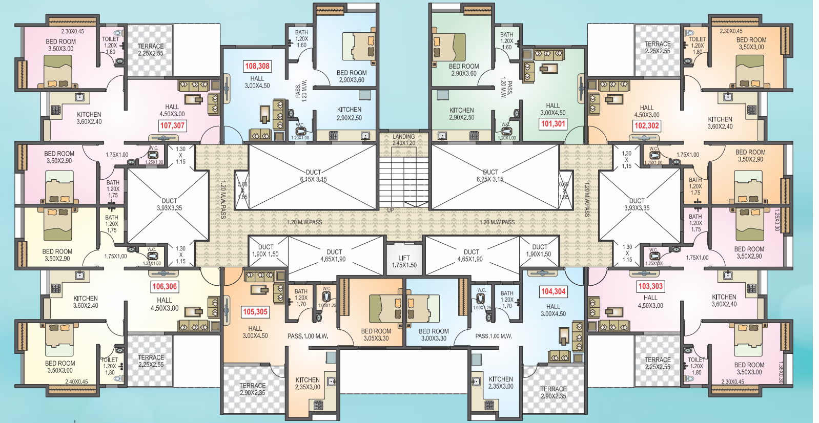
1ST & 3RD FLOOR PLAN
