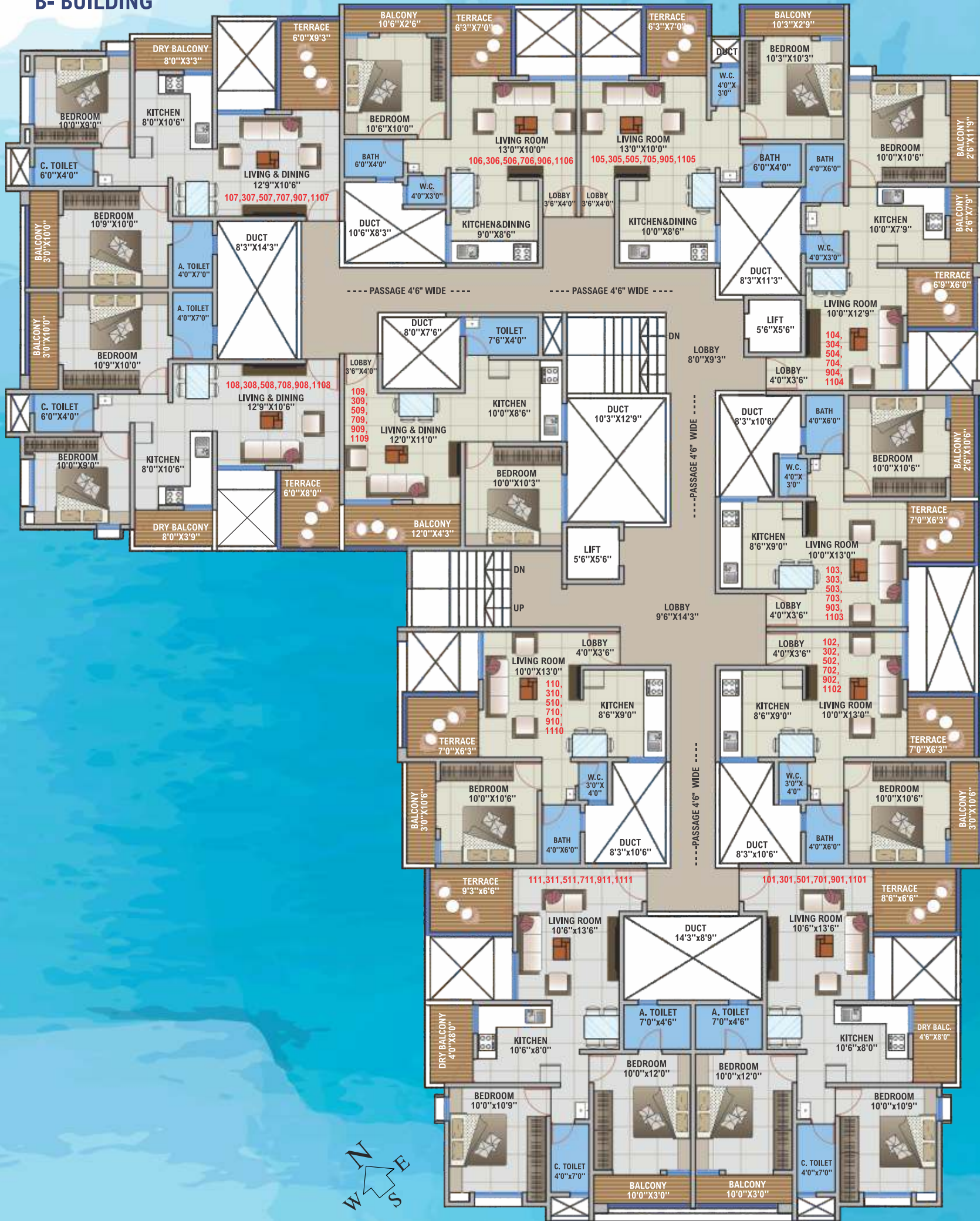
FIRST, THIRD, FIFTH, SEVENTH, NINTH AND ELEVENTH FLOOR PLAN
